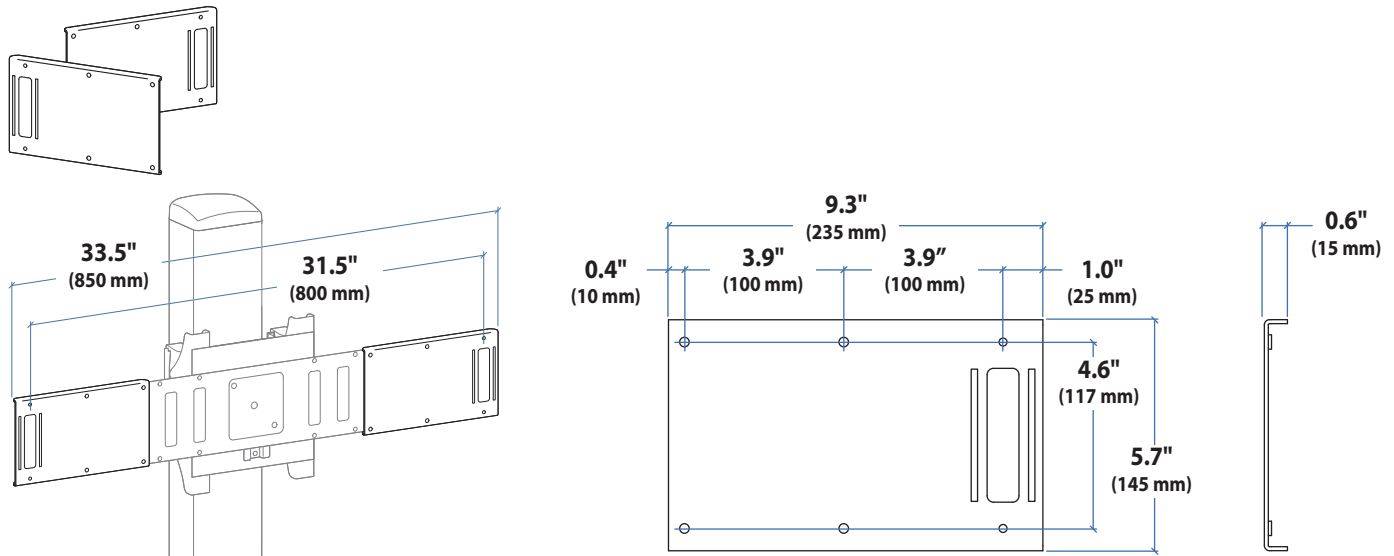
800 mm Expansion Kit
