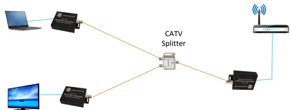
Multi-Drop Connection
