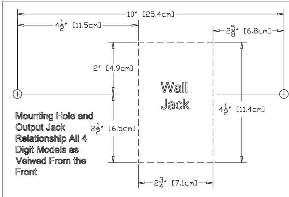
Figure 5: Mounting Template for 4-Digit Clocks
