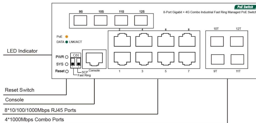
Figure 3-1 Front panel of 20117402
