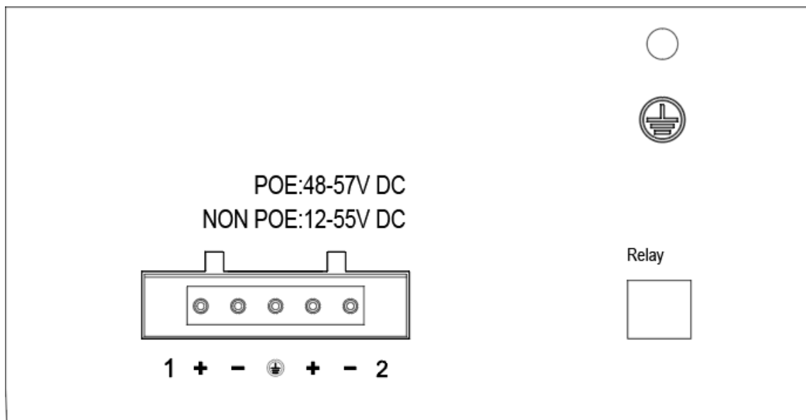
Figure 3-2 20117402 Switch side panel
