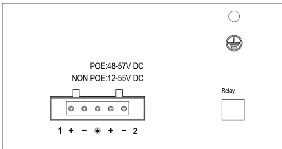
Figure 3-2 20117399 Switch side panel
