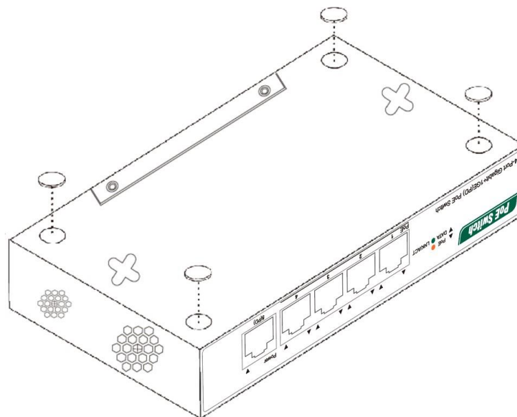
Figure 3-1 Desktop Installation Diagram
