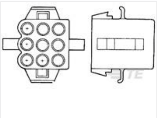
TE Part #1-480672-0 09P .140 MNL PLUG PM NAT
